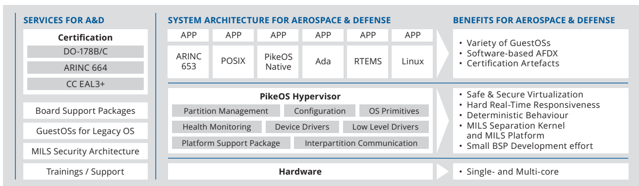
Figure 1: Scheme of an Aerospace & Defense System with PikeOS Architecture
